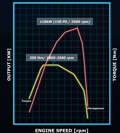
1.9L R24E-TC ENGINE
