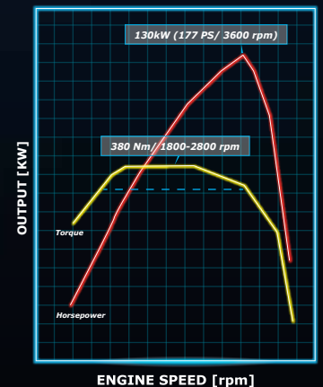
3.0L 4JJ1-TCX ENGINE
